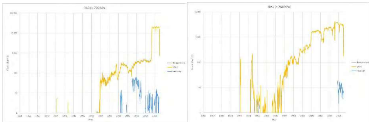
Figure 27. Number of aircraft observations in RA3 (left) and RAI (right) JMA Archive
