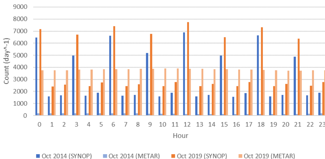
Figure 13. Average counts of surface air-temperature observations over land for each hour of the day for October 2014 and 2019 from the JMA operational receipt of data after duplicate removal and elimination of sub-hourly data
