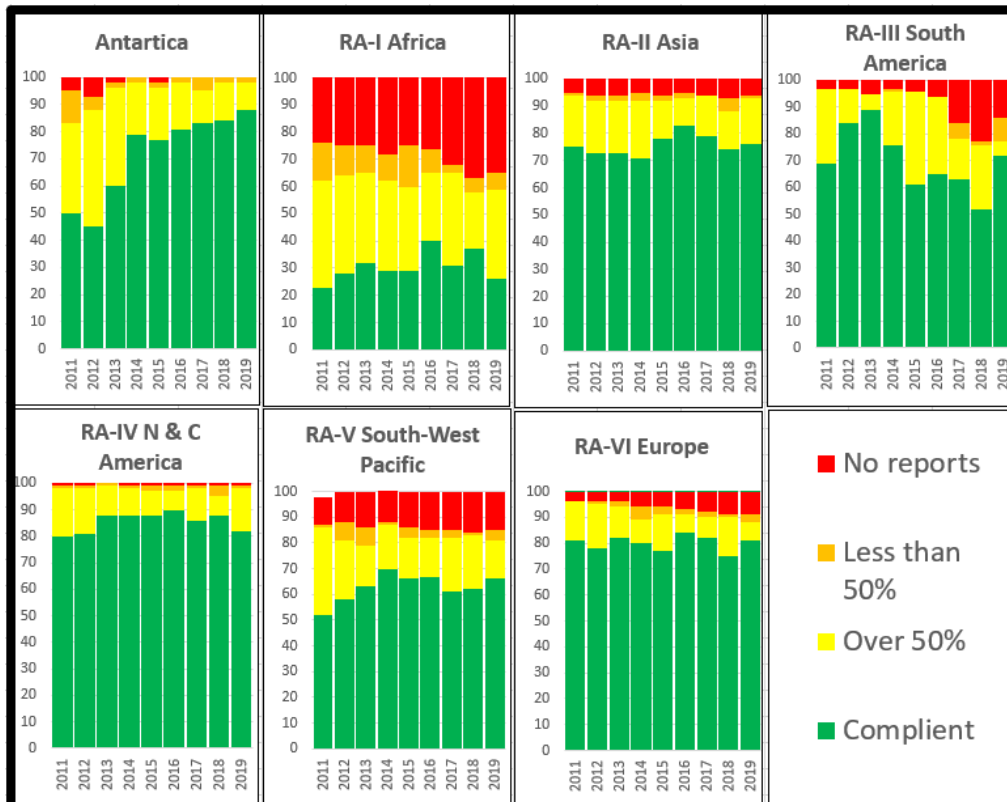
Figure 31. GSN NCEI CLIMAT availability monitoring statistics 2011-2019
